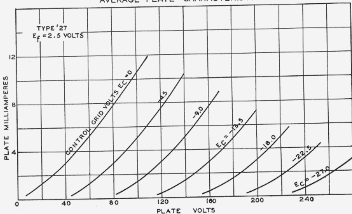
AVERAGE PLATE CHARACTERISTICS
